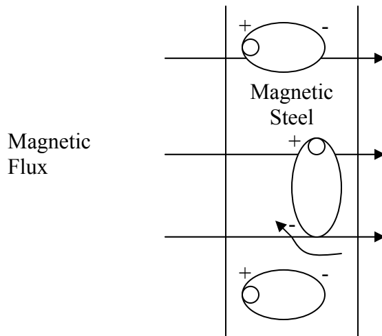
Figure 4: Magnetic Dipoles
