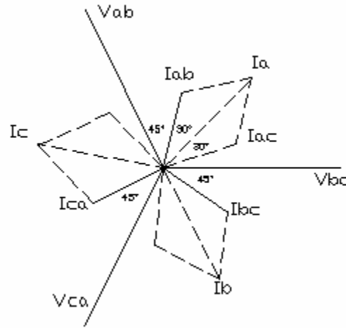
Figure 5: Good Winding Balanced Wye
