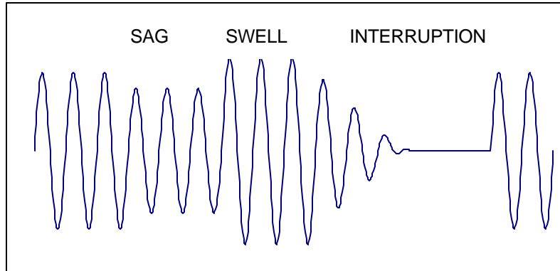
Figure 4. RMS Variations
