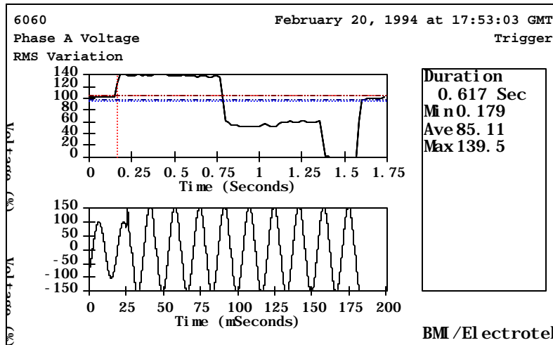
Figure 5. Swell, Sag and Interruption in Same Event
